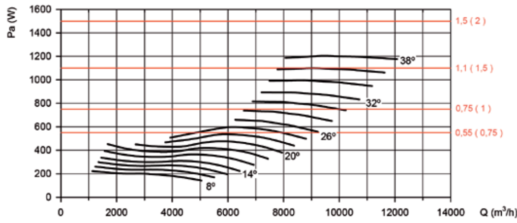
Absorbed power
