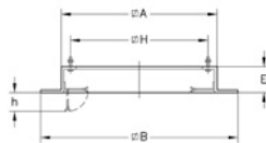
MS. Support frame for easier mounting
