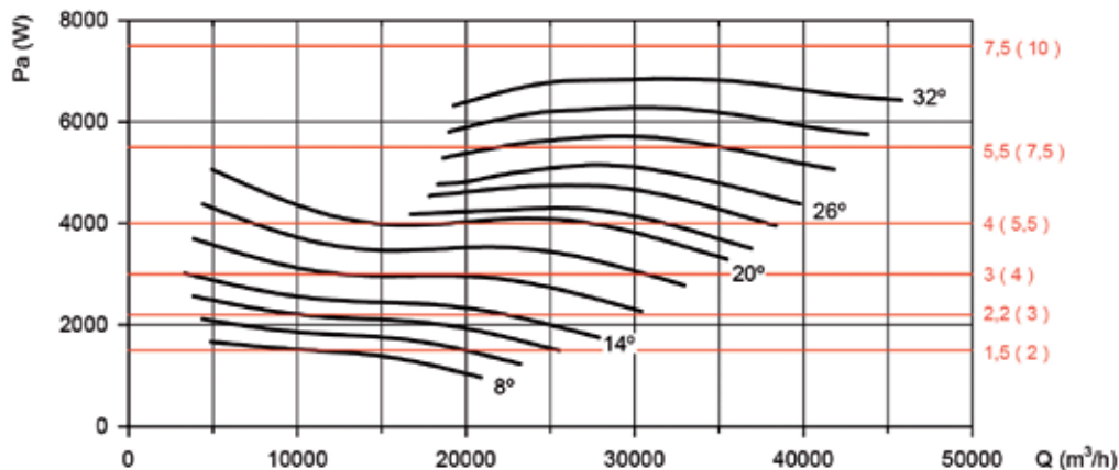
Absorbed power
